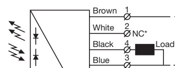
SMP / SMPF / SMRR 7600 (load as PNP)
