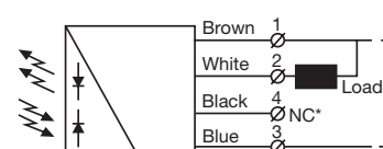
SMP / SMPF / SMRR 7600 (load as NPN)
