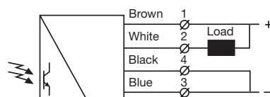
SMR 640x / 650x (load as NPN)
