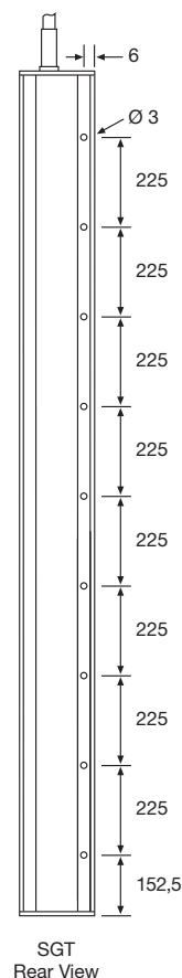
SGT Rear View
