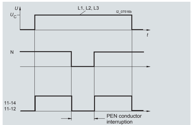
Timing interval of 5TT3 410 N conductor monitors
