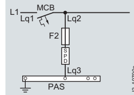
a) Protection of the SPD over miniature circuit breakers
