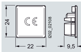
5ST3 750-0HG
