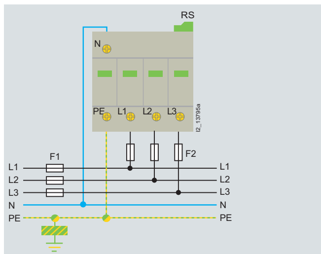
5SD7 424-, for TN-S/TT systems
