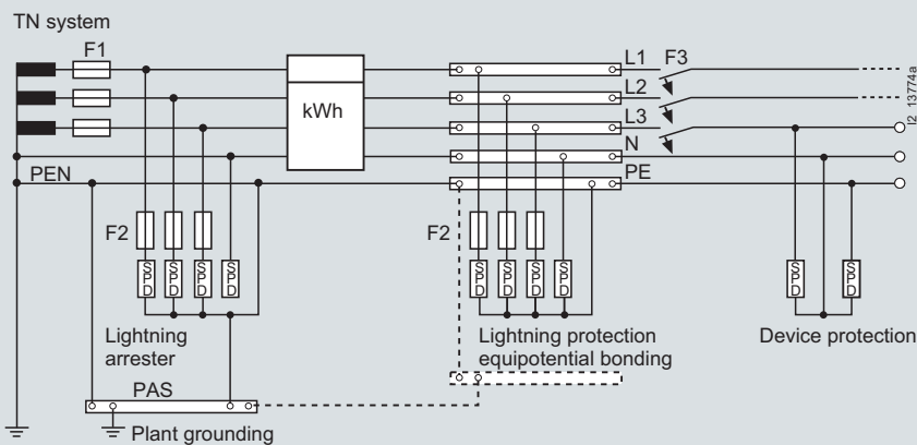
TN-S system
