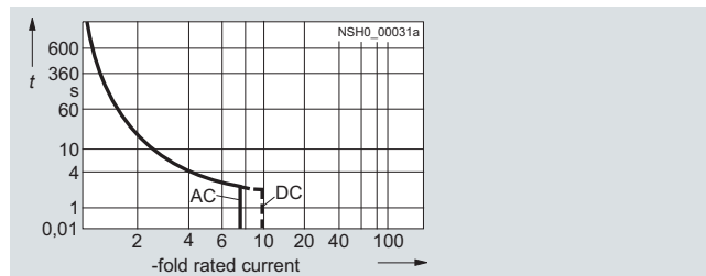
Tripping characteristics of combined overload and short-circuit releases at an ambient temperature of 40 °C
