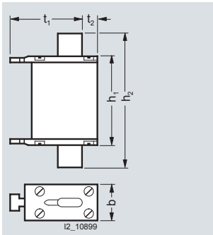
Size 000 to 3
