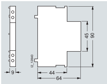
5TT5 910-0 5TT5 910-1
