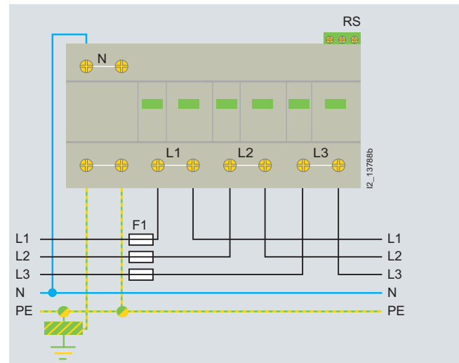
5SD7 444-1 for TN-S/TT systems
