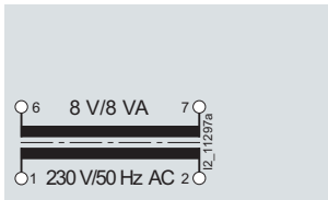
4AC3 408
