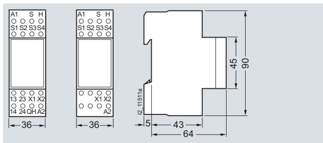
5TT3 460
