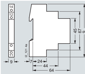
5TT4 90.
