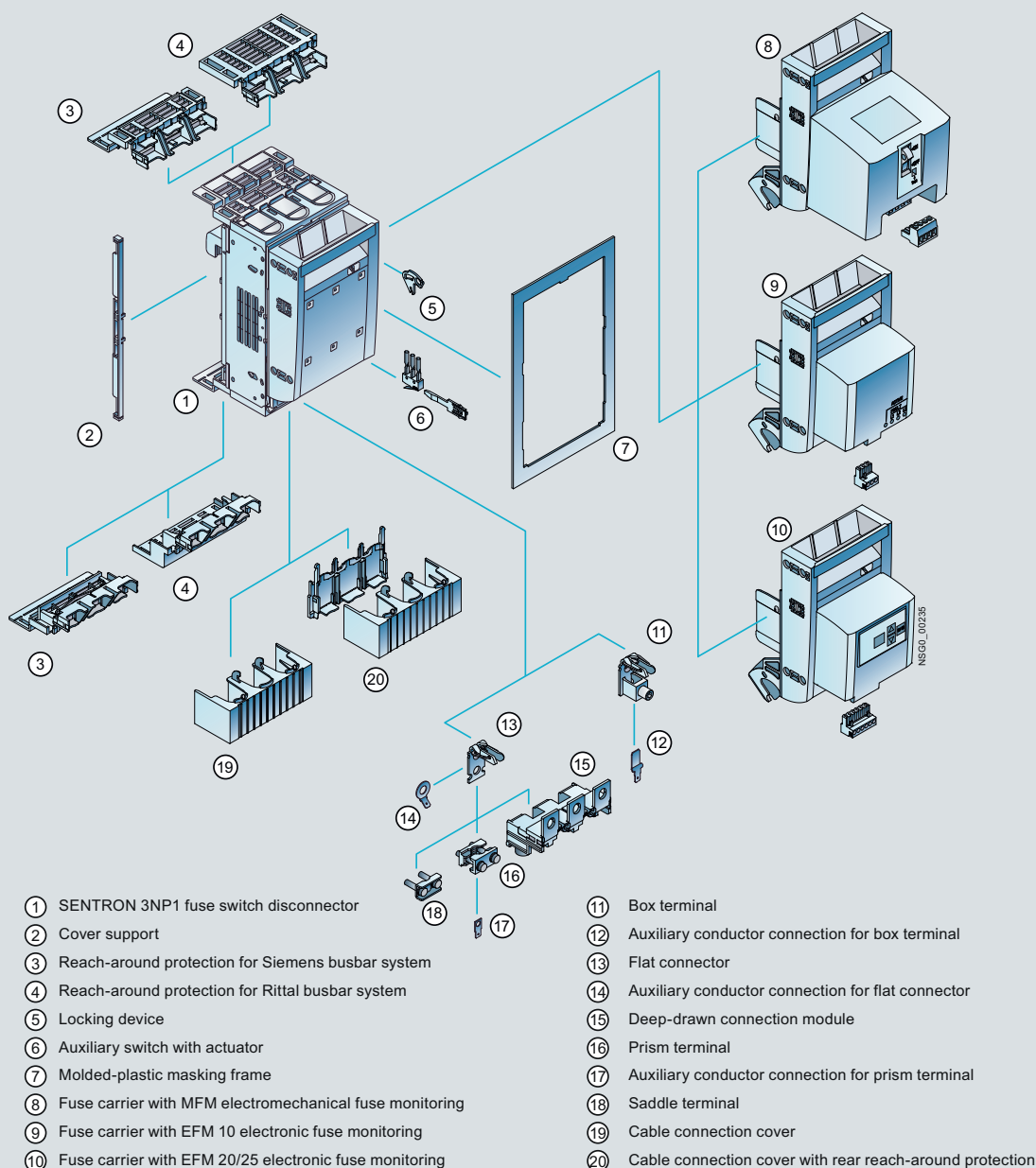
3NP1 fuse switch disconnector
