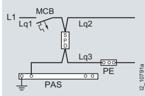
a) Protection of the SPD over miniature circuit breakers
