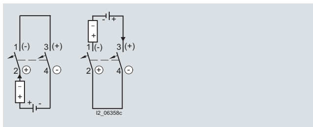
Miniature circuit breaker, two-pole for single-pole tripping Non-grounded system (left: bottom infeed, right: top infeed) Rated voltage of miniature circuit breaker: 440 V
