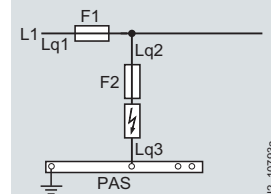
a) Protection of the SPD over fuses
