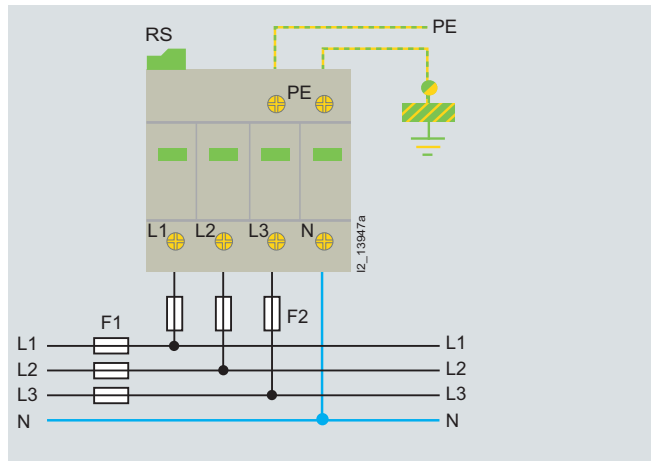
5SD7 464-, for TN-S/TT systems
