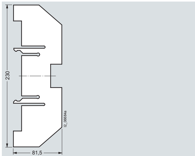
For LV HRC bus-mounting bases in tandem design 3NX2 031
