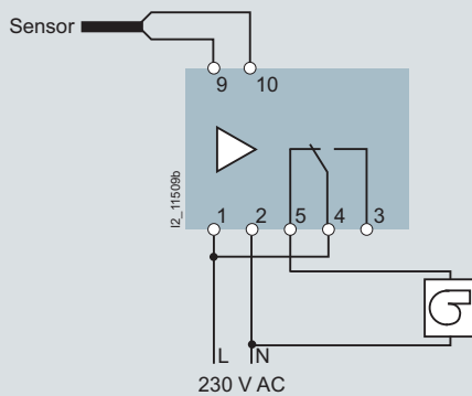
7LQ2 0
