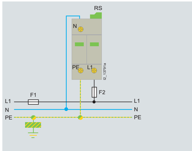
5SD7 422-, for TN-S/TT systems
