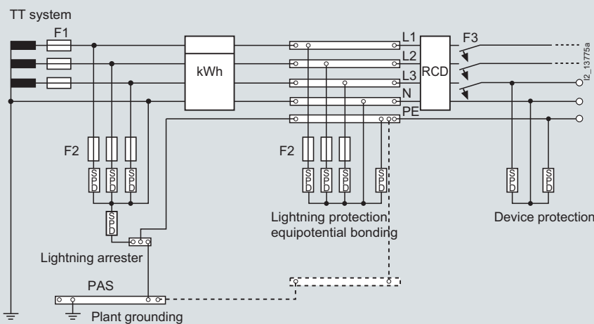
TT system
