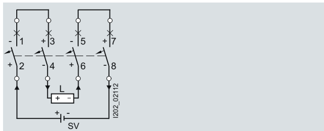
Miniature circuit breaker, four-pole for two-pole tripping Non-grounded system (bottom infeed) Rated voltage of miniature circuit breaker: 880 V
