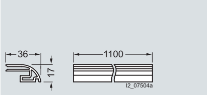
5SH3 528
