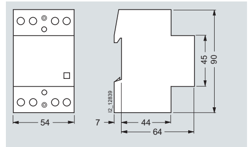
5TT5 84.-0 5TT5 84.-2 5TT5 85.-0 5TT5 85.-2
