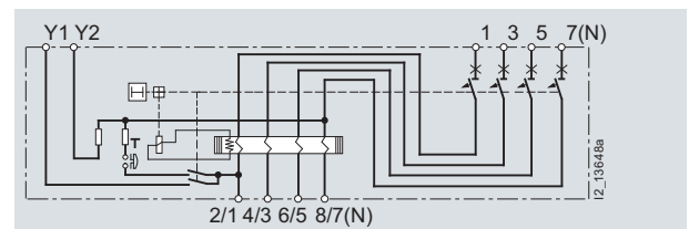
4P, 125 A
