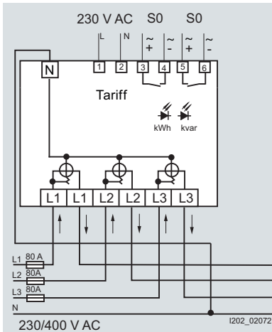
7KT1 543, 7KT1 545, three-phase connection
