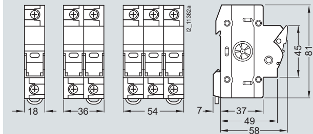
3NC1 09.
