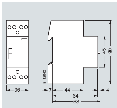
5TT5 83.-6 5TT5 83.-8
