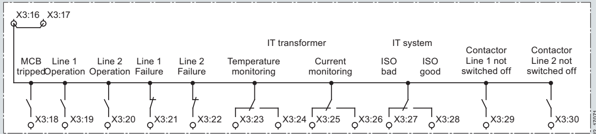
Terminal diagram for connection of 7LQ3 361 and 7LQ3 362 switchover devices to the central building control system devices
