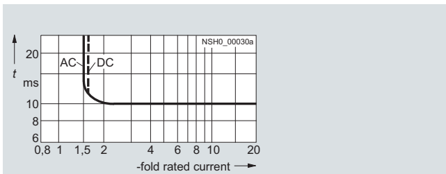
Tripping characteristics of short-circuit releases
