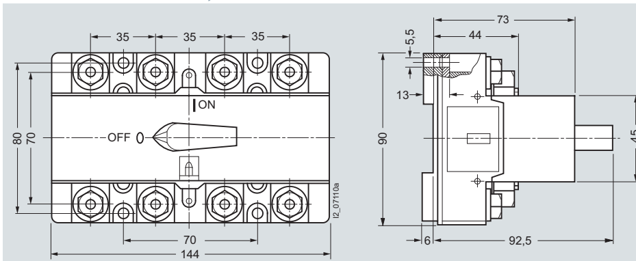
5TE1 switch disconnectors, 160 A and 200 A
