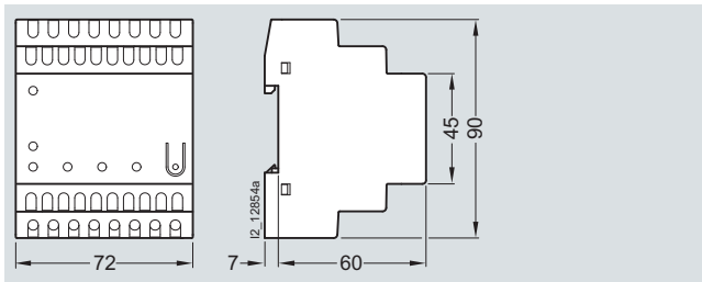
5TT7 120
