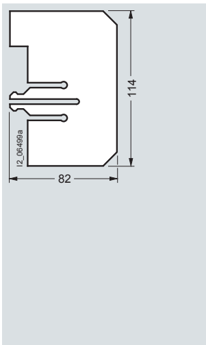
Phase barriers 3NX2 027
