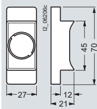
5SH5 251 (A4) and 5SH5 253 (A10)
