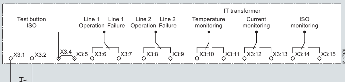
Terminal diagram for connection of 7LQ3 361 and 7LQ3 362 switchover devices to test signaling device (e. g. 7LQ3 356 and 7LQ3 357 test and signaling panels)
