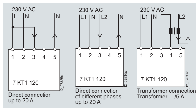
Digital ammeters
