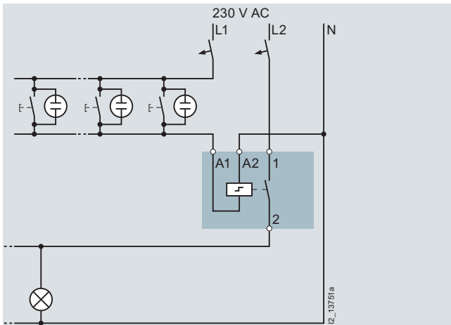
Single-phase lighting circuit with 230 V AC actuation, e. g. in office buildings
