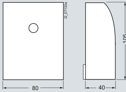
5TT3 303
