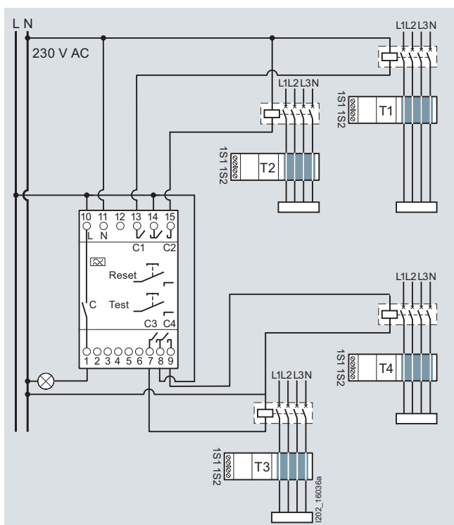
RCM digital, 4 channels, 5SV8 200-6KK, Shunt trip (ST)
