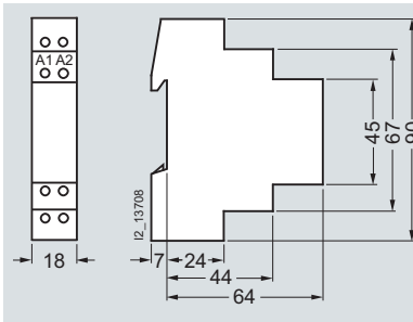
5TT4 920
