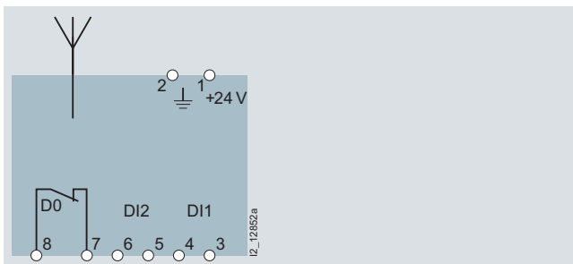
5TT7 120
