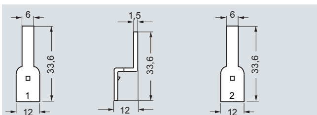
5ST3 510-0
