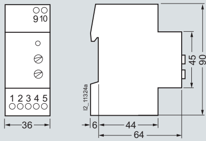
7LQ2 0
