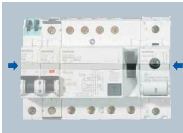
A labeling concept for all devices – the labeling fields are at the same height on all devices
