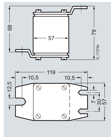
3NC7 3...-2
