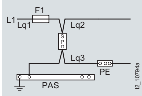
a) Protection of the SPD over fuses
