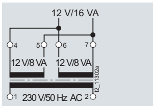
4AC3 616, parallel switching
