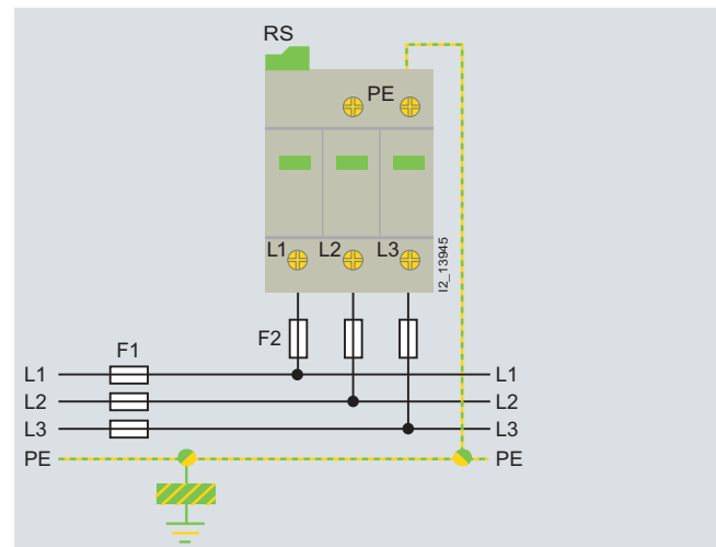
5SD7 473- for IT systems
