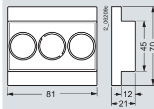
5SH5 252 (A5) and 5SH5 254 (A11)
