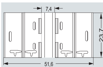
5ST3 508-0
