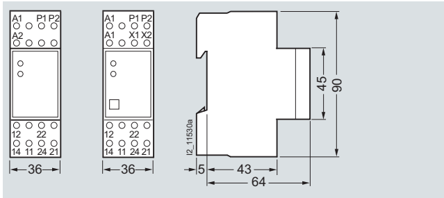
5TT3 431
