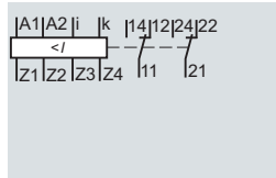
5TT6 114
