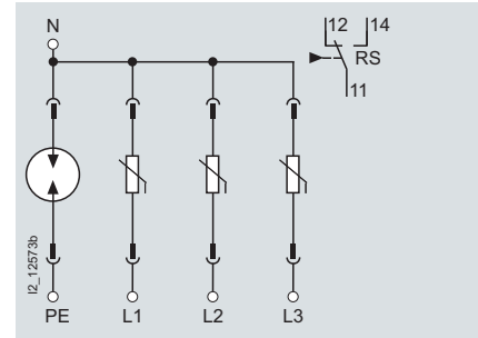
4P 5SD7 424-0 without RS 1) 5SD7 424-1 with RS 1)
