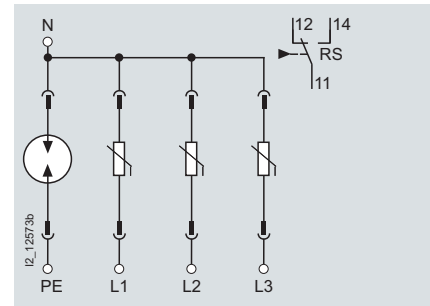
5SD7 464-0, 5SD7 485-0 without RS 1) 5SD7 464-1, 5SD7 485-1 with RS 1)
