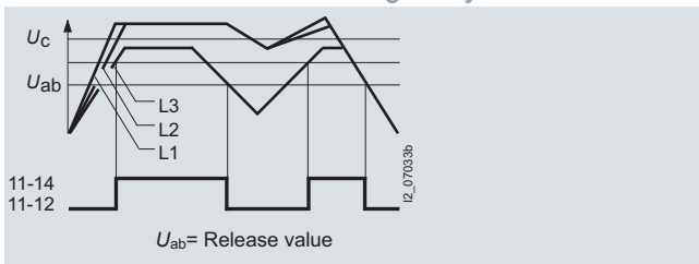
Timing interval of 5TT3 400 ... 5TT3 406 undervoltage relays
