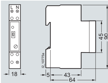
5TT3 171
