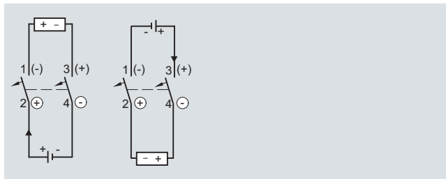
Miniature circuit breaker, two-pole for two-pole tripping Non-grounded system (left: bottom infeed, right: top infeed) Rated voltage of miniature circuit breaker: 220 V
