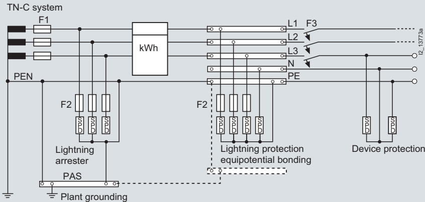
TN-C system
