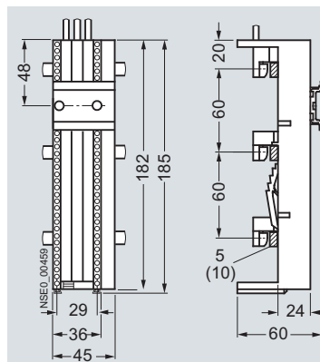
8US12 51-5CM47
