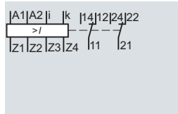
5TT6 113
