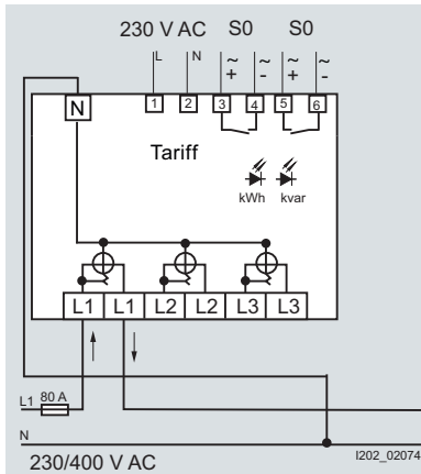
7KT1 543, 7KT1 545, single-phase connection
