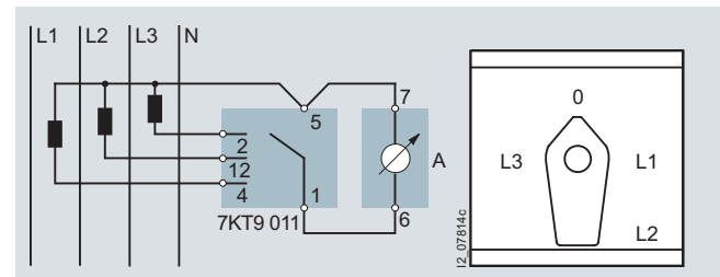
Ammeter switching
