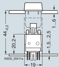
Illuminated pushbutton with solder pin connection
