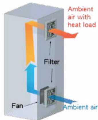
Fig.3 Pressure System
