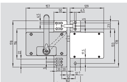
AZM 415-STS30
