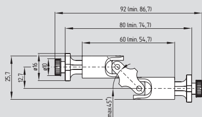
Universal joint K1
