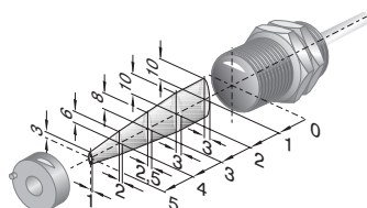
Enabling zone
