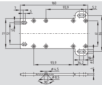
Adapter plate kit
