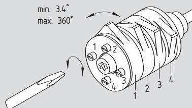
Teardrop cam with front setting -1600-1
