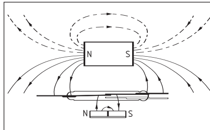
Combined effects of magnetic field lines using a change-over contact and a N-S magnet.
