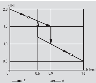
Force-Travel on plunger
