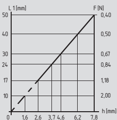
Force-Travel on lever bearing II
