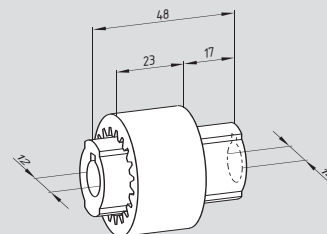
Bowex coupling
