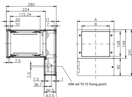
Enclosure with connection compartment / 19" mounting frame with transparent cover
