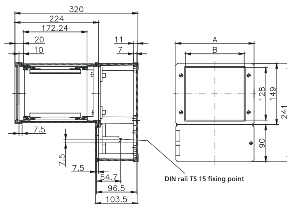
Enclosure with connection compartment / 19" mounting frame with transparent cover
