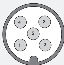
M connector (5 pin) M12 A coded solder side view FV
