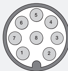
M connector (8 pin) M12 A coded solder side view FV
