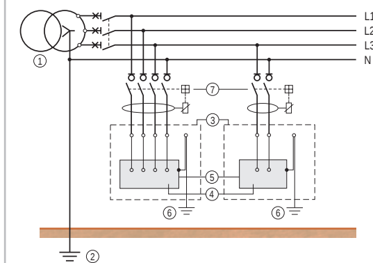
TT wiring diagram
