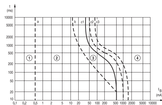
Time / current zones of effects of AC current (15Hz to 100 Hz) on persons (fig. 1)
