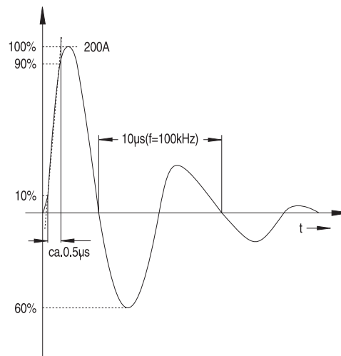
Curve 0.5 \mu s - 100 kHz - 200 A - EN/IEC 61008/61009
