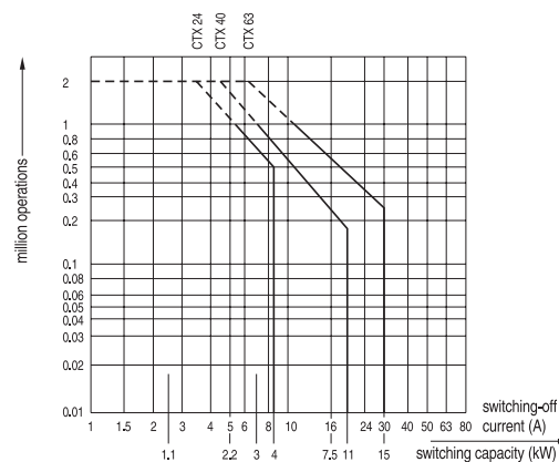
fig.8B Endurance curve (Operations vs. switching-off current (kW)) AC-3/400 V 3- for CTX 24, 40, 63 AC-3/230 V 1- for CTX 20
