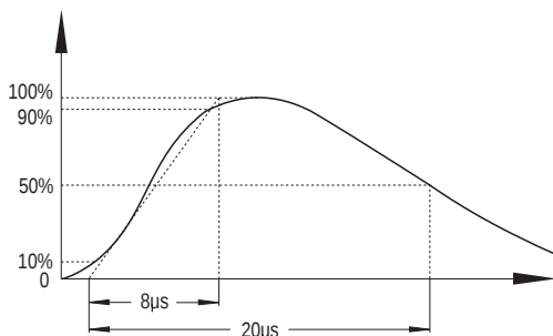
Curve 8/20 \mu s
