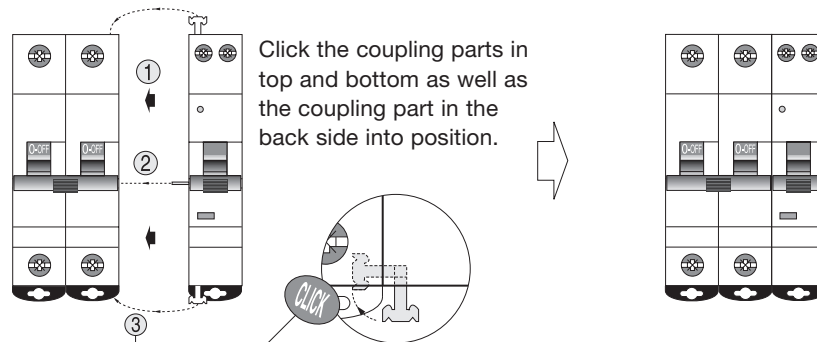
fig.1 To couple on the right-hand side
