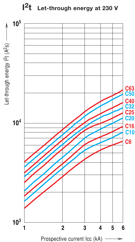
G45 Curve C 2P
