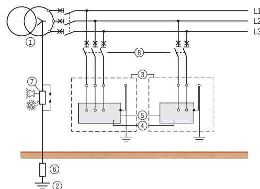
IT wiring diagram
