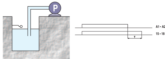
fig.3 Delay On and Off (PLT OO)
