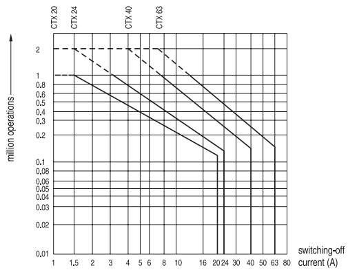
fig.8A Endurance curve (Operations vs. switching-off current) AC-1/400 V 3- for CTX 24, 40, 63 AC-1/230 V 1- for CTX 20
